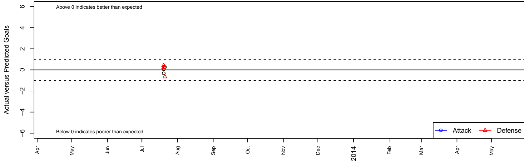
Hawaii Rush 02 Nike B01 Dots are actual minus expected GF (blue circles) and GA (red triangles). Blue line is smoothed change in attack strength. Red is smoothed change in defense strength.
